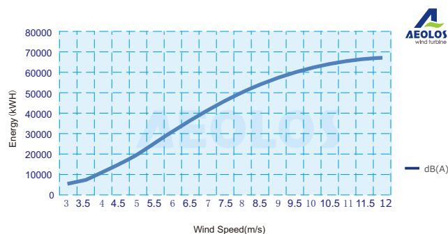
AEP of 10kW wind turbinr
